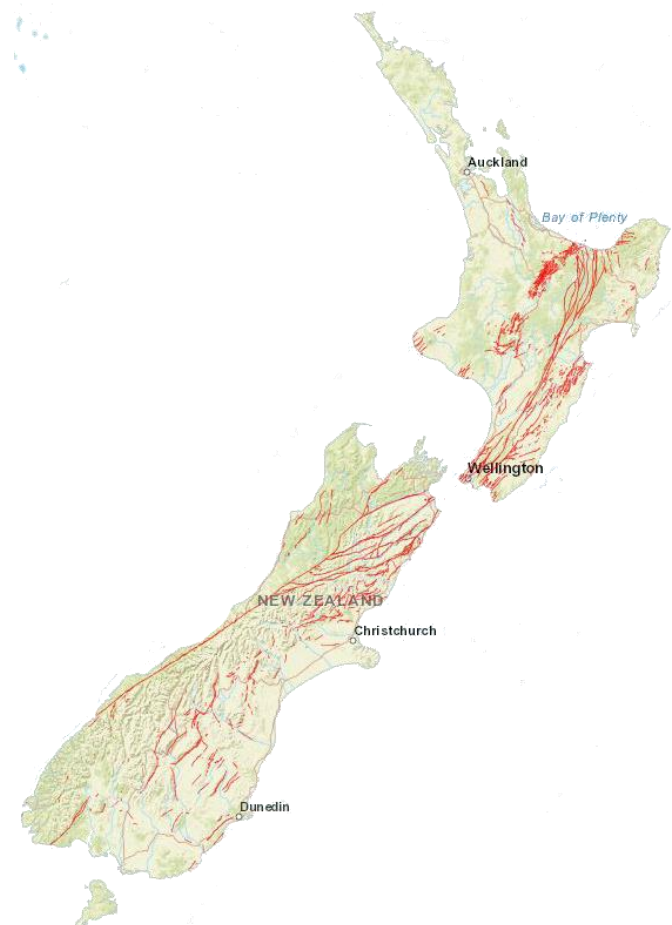
Figure 2-7: Active Fault Database (GNS)
