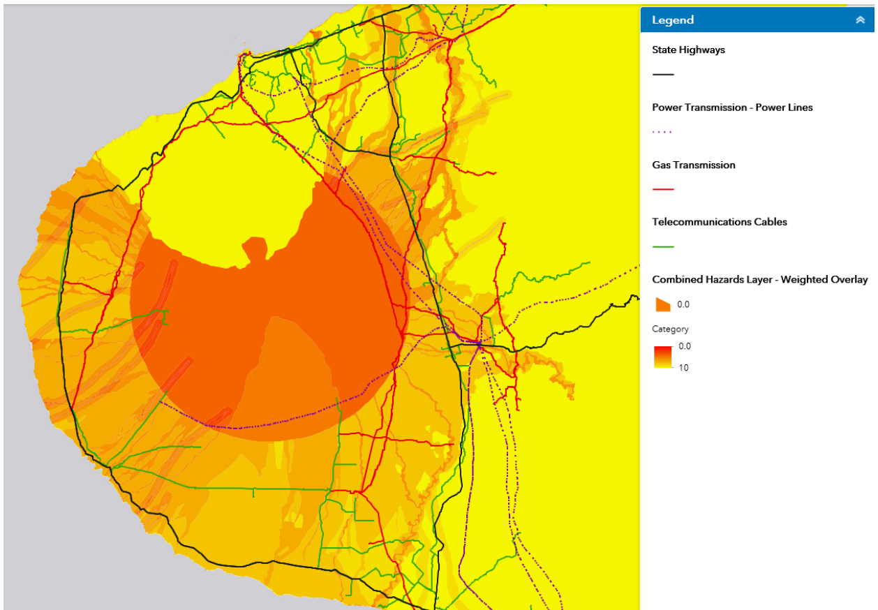
Figure 2-4: 'Combined Hazards' (Volcanic Hazards of Taranaki: 1996. Neall, VE; Alloway B.V., Massey University and Department of Soil Science Occasional Report.
