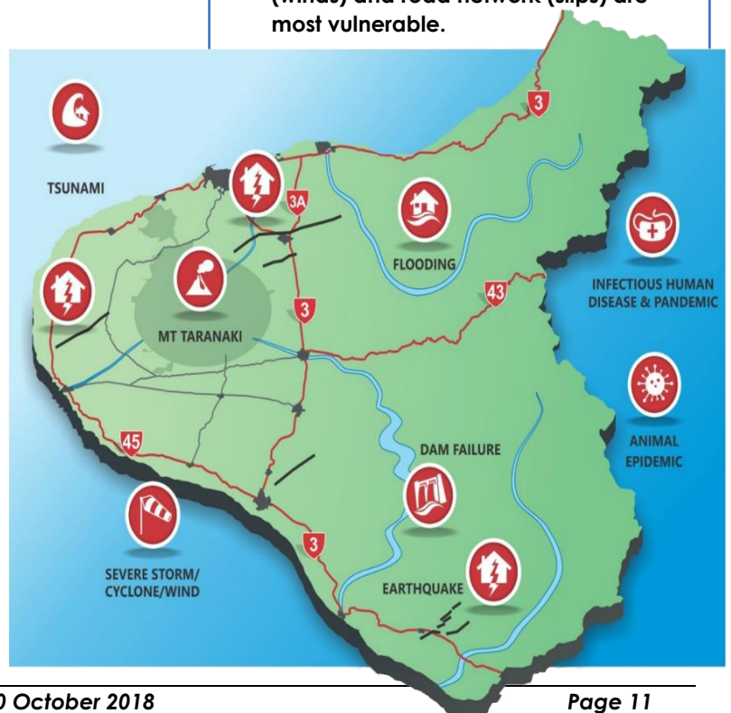
Figure 2-1: Taranaki Hazards (Source: CDEM Group Plan for Taranaki 2018-23)
