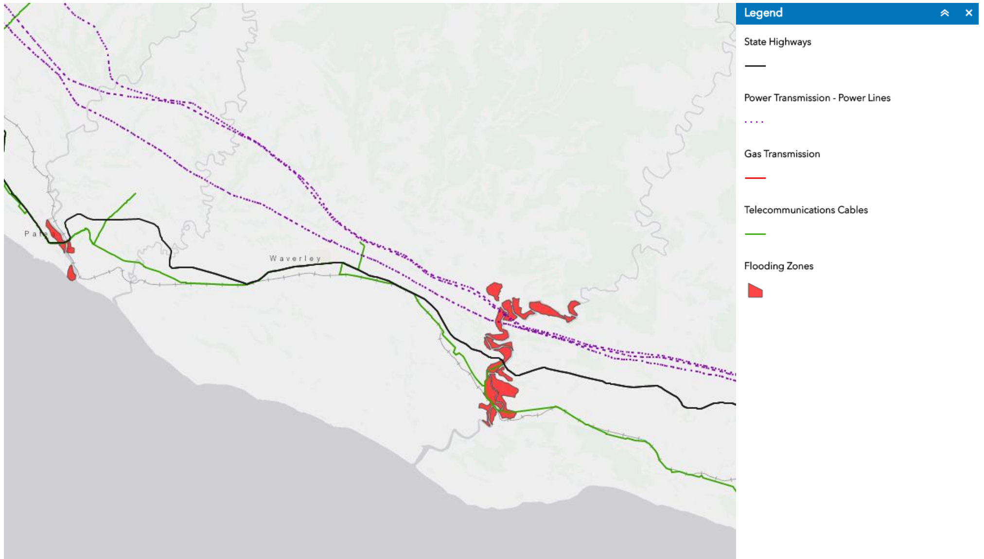
Figure 2-12: Flood Inundation Areas – South Taranaki area
