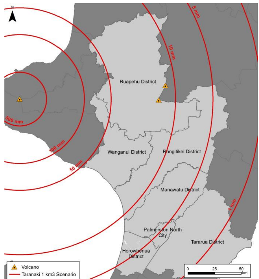
Figure 2-3: Volcanic Ash Modelling, Mt Taranaki (westerly, 1:2,500 yr event). Source: GNS for Manawatu-Wanganui Lifelines Project 2016.
