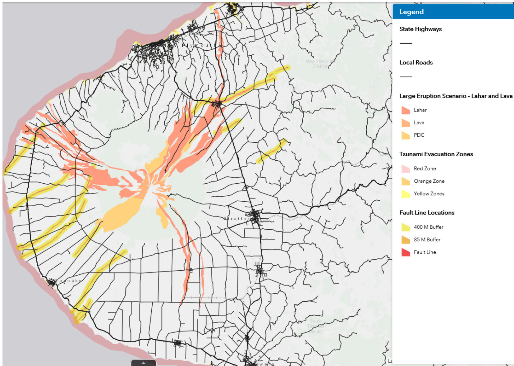
Figure 3-6: Road Network shown with Seismic, Near-Source Volcanic and Tsunami hazard layers
