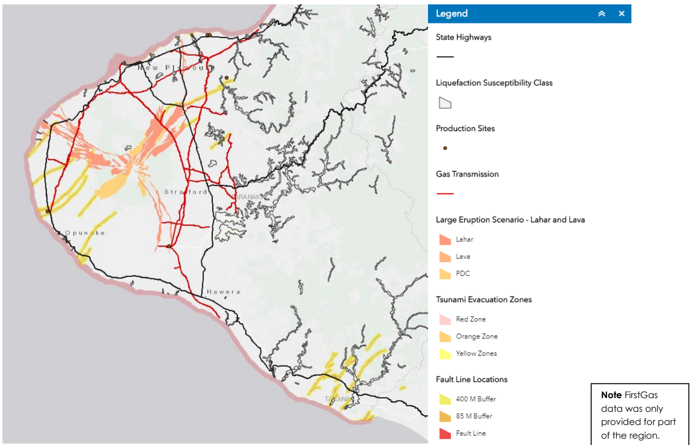
Figure 3-4: Gas Transmission shown with Seismic, Near-Source Volcanic and Tsunami hazard layers
