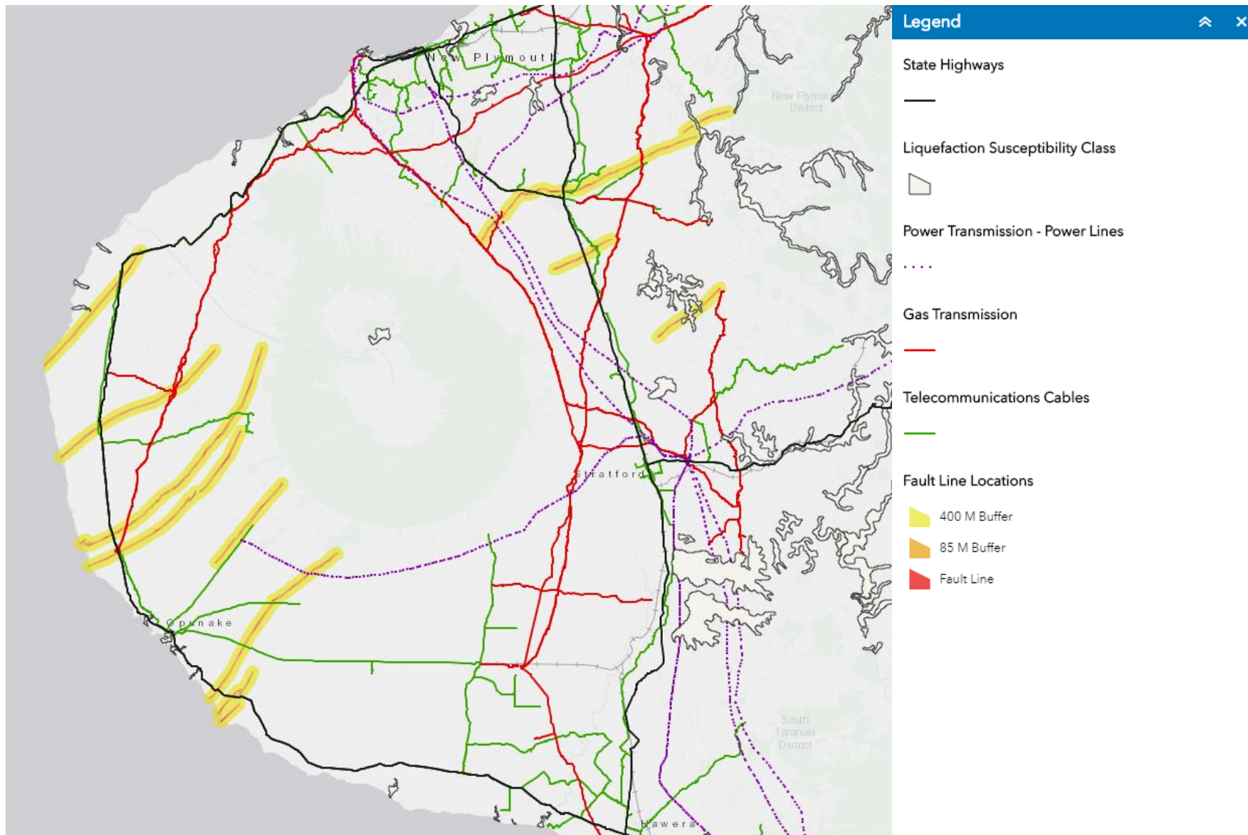
Figure 2-8: Fault Lines and Liquefaction Susceptibility
