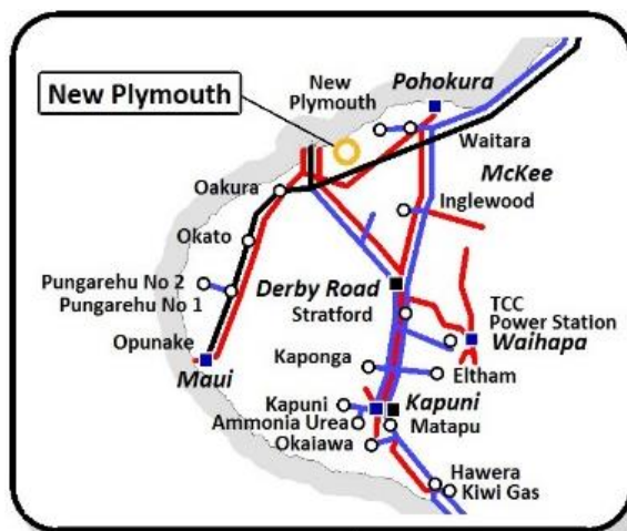
Figure 3-3 First Gas Network in Taranaki
