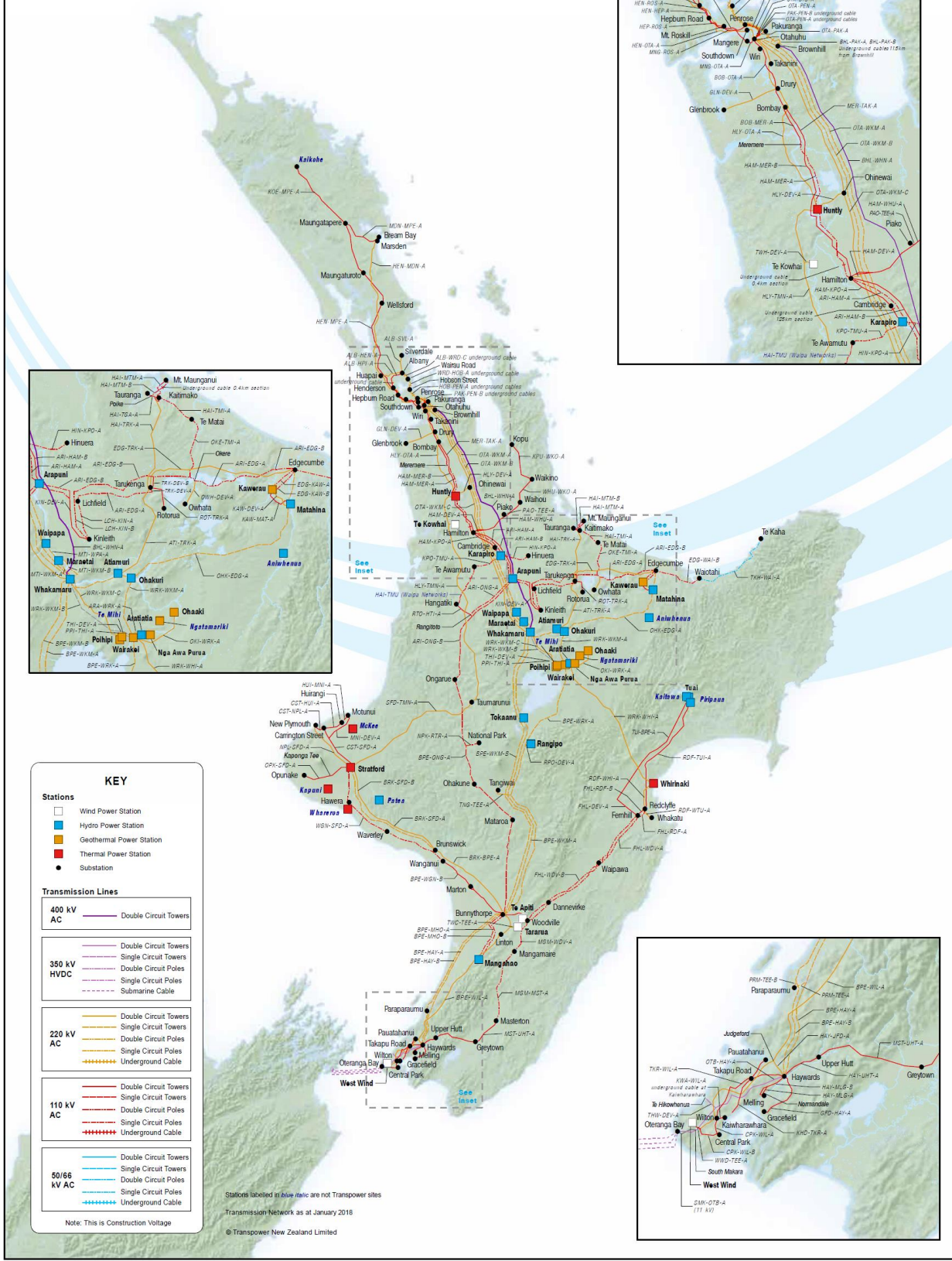
Figure 3-1: North Island National Grid
