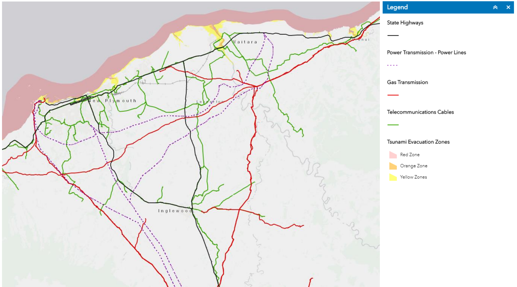
Figure 2-10: Tsunami Evacuation Zones
