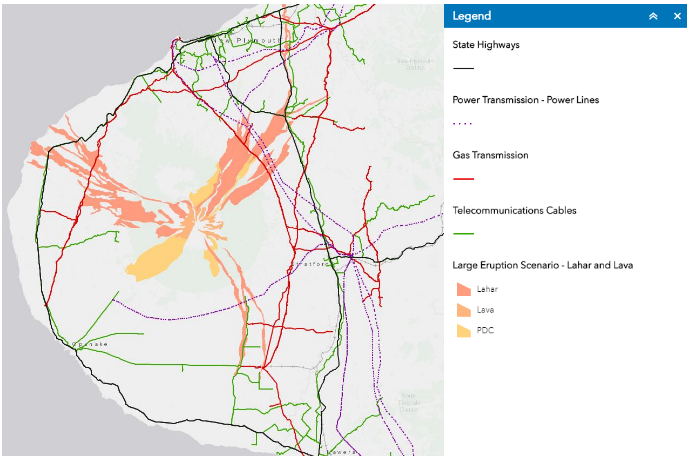
Figure 2-5: Large Eruption Scenario – Lahar, Lava Flows (Source ...)
