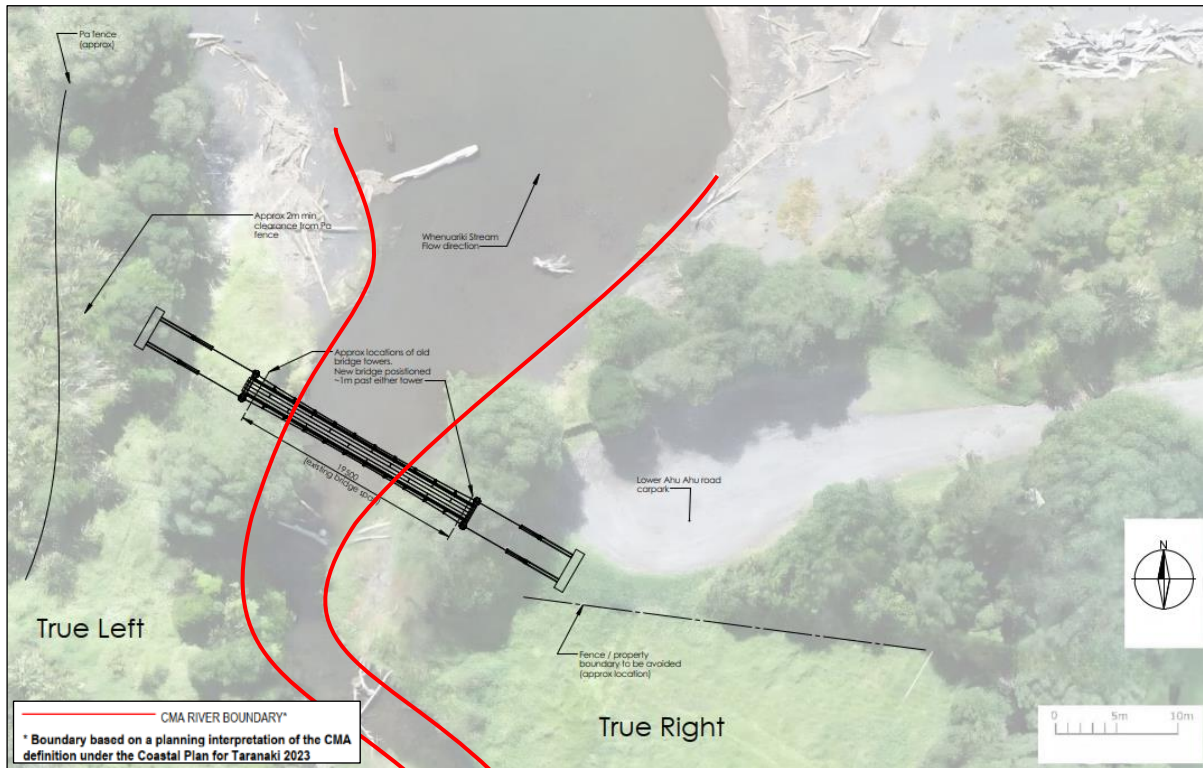
Figure 1.2: Ahu Ahu Bridge concept design [Updated to include planning interpretation of CMA boundary at Whenuariki Stream].
