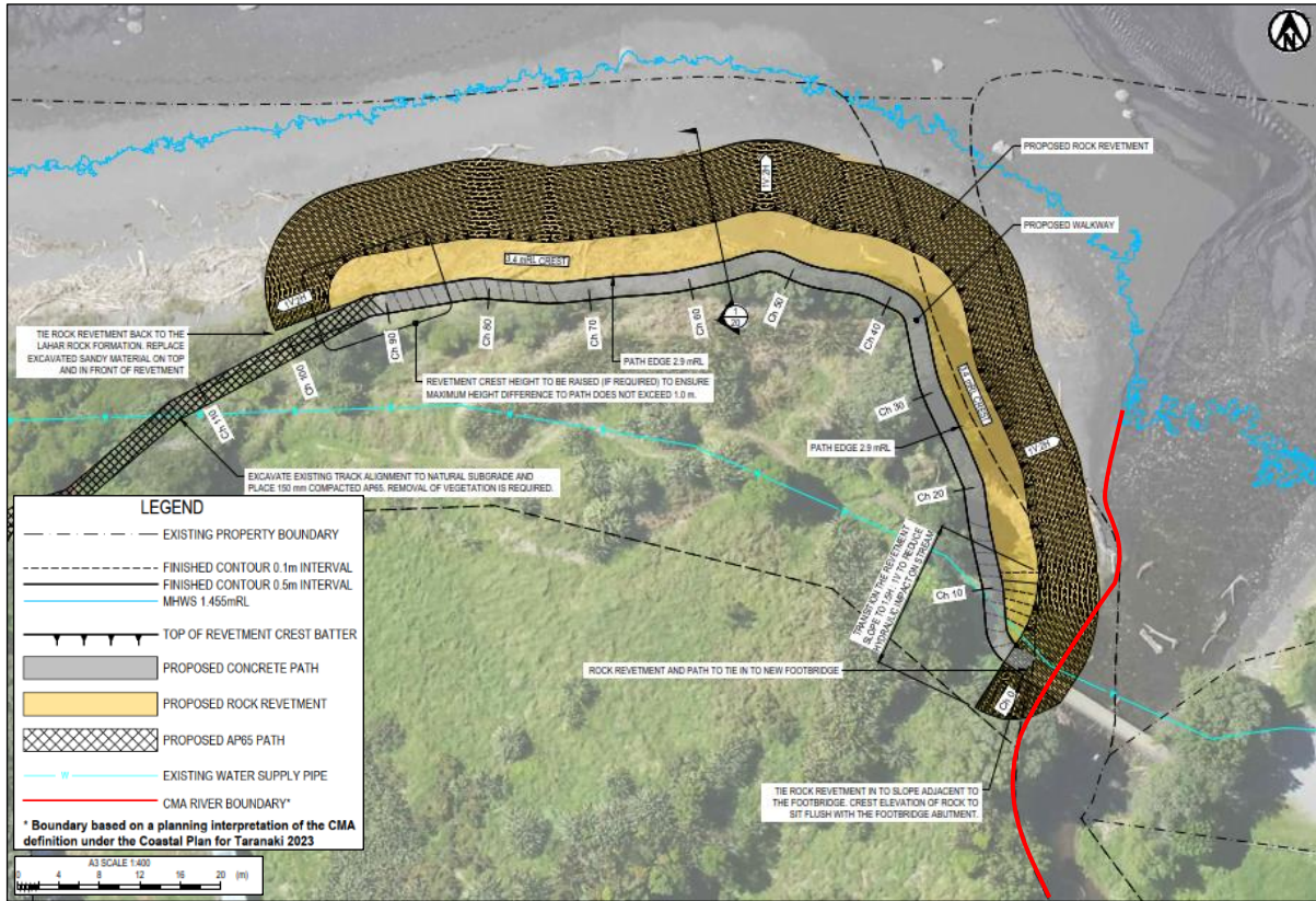
Figure 1.1: Shared pathway and revetment crest proposed concept design [Updated to include planning interpretation of CMA boundary at Whenuariki Stream].
