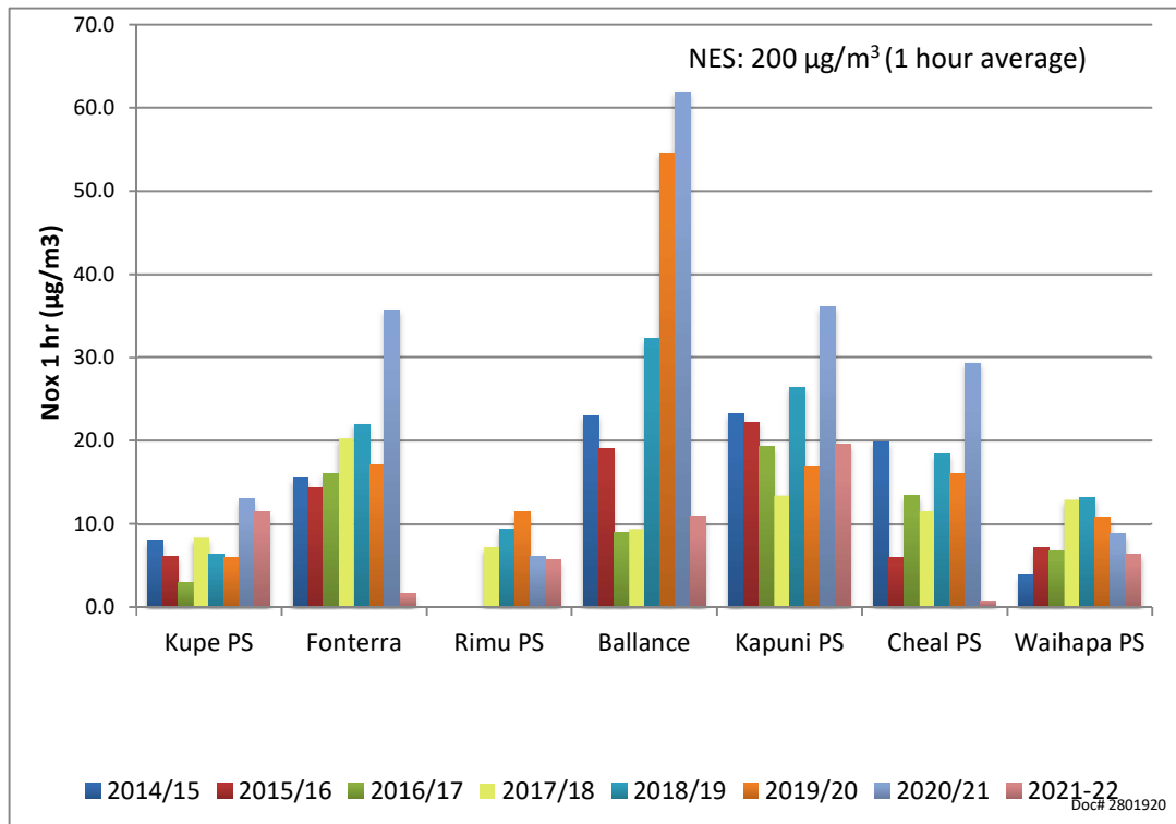
Figure 2 Average NOx levels at seven Southern surveyed locations throughout the region (year 2021-2022)
