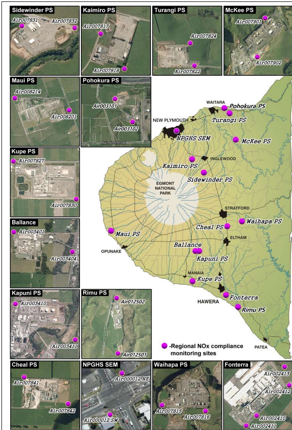
Figure 2 NOx monitoring sites in Taranaki Region, 2021-2022
