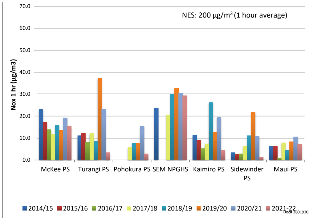
Figure 1 Average NOx levels at seven Northern surveyed locations throughout the region (year 2021-2022)
