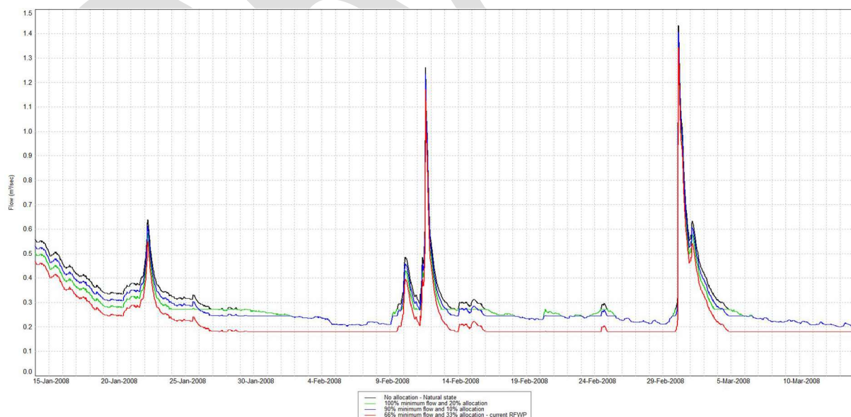
Figure 8 Example of a 'small stream' with no abstraction (natural state)(black), 100% minimum flow, with 20% allocation(green), 90% minimum flow, with 10% allocation(blue) and current RFWP rules of 66% minimum flow and 33% allocation(red).
