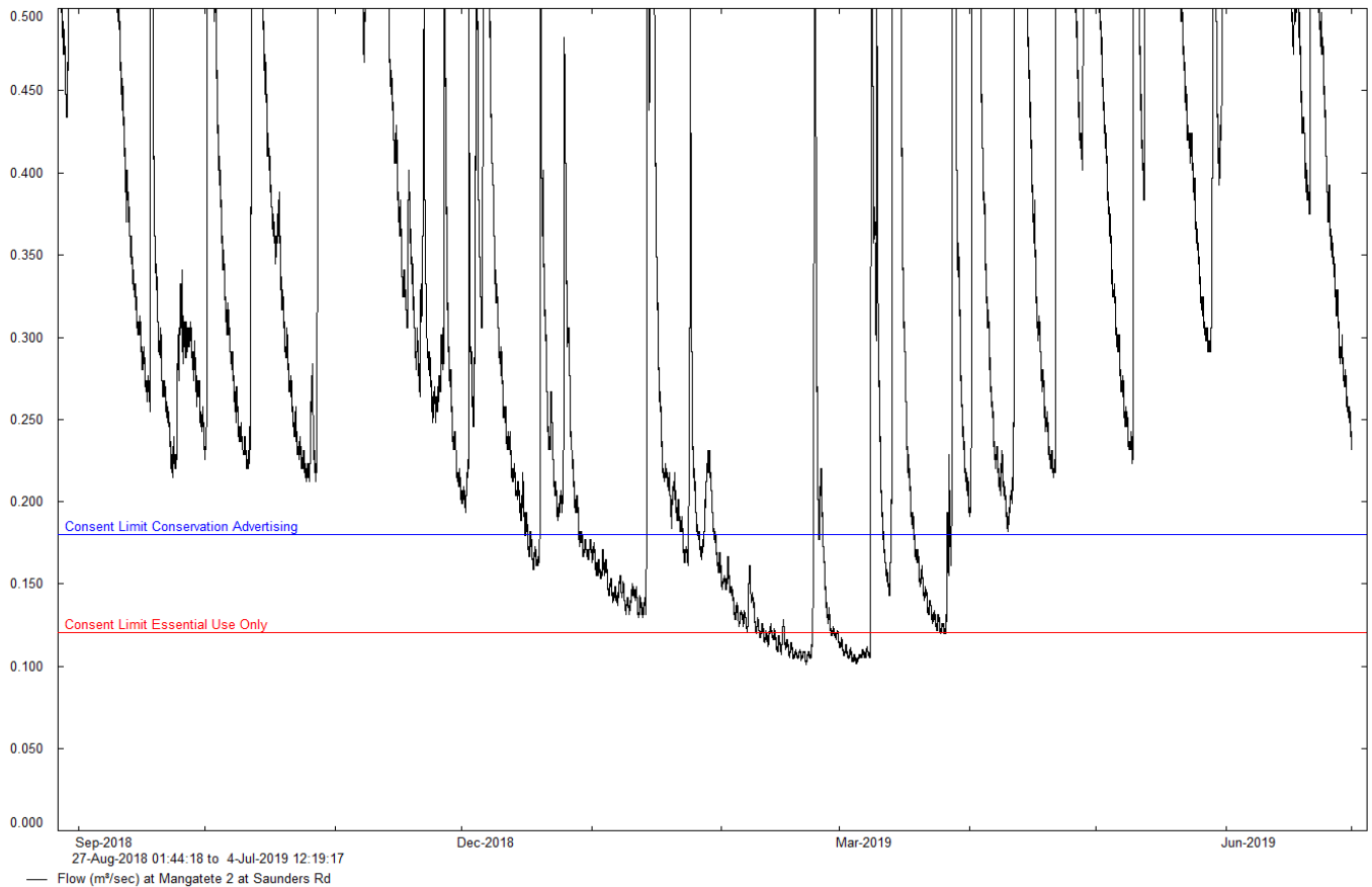
Figure 2 Residual flow in the Mangatete Stream during the dry season
