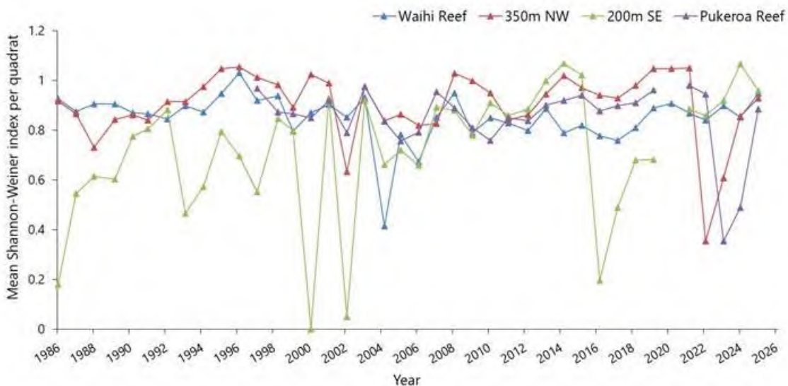
Figure 6 Mean Shannon-Weiner Indices per quadrat for summer surveys (1986-2025)
