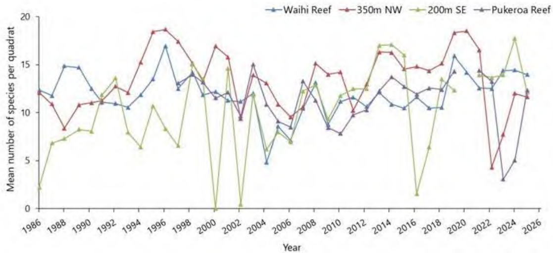
Figure 5 Mean number of species per quadrat for summer surveys (1986-2025)
