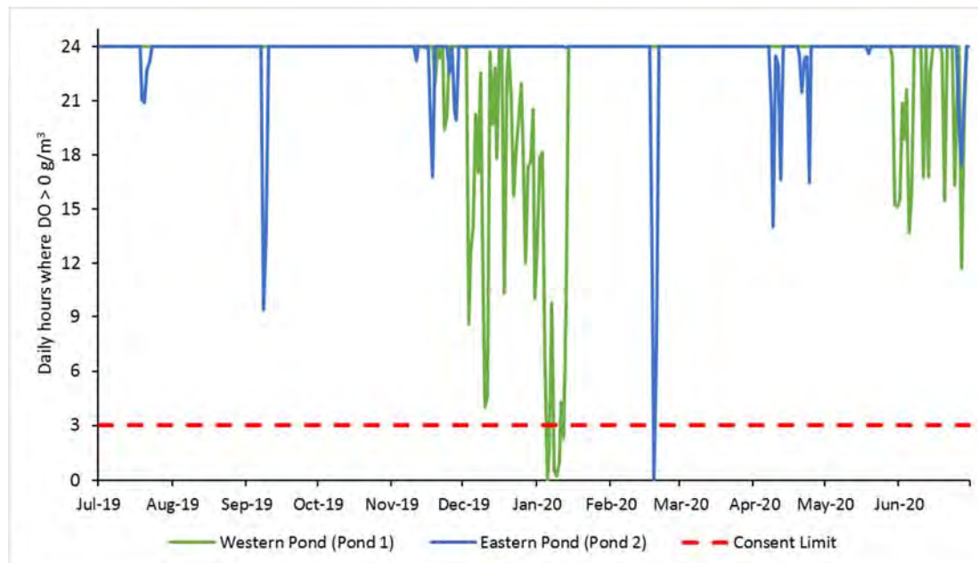
Figure 2 Daily hours where DO is greater than 0 g/m 3 in Pond 1 and 2
