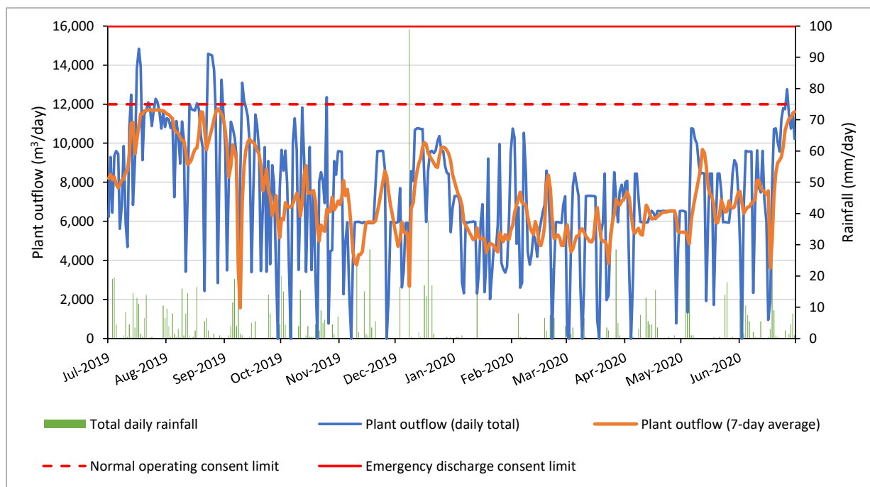
Figure 3 Daily discharge volumes ( \text{m}^3/\text{day} ) from the HWWTP and daily rainfall data (mm) from a Council rainfall station located approximately 5 km east of the site (2019-2020)
