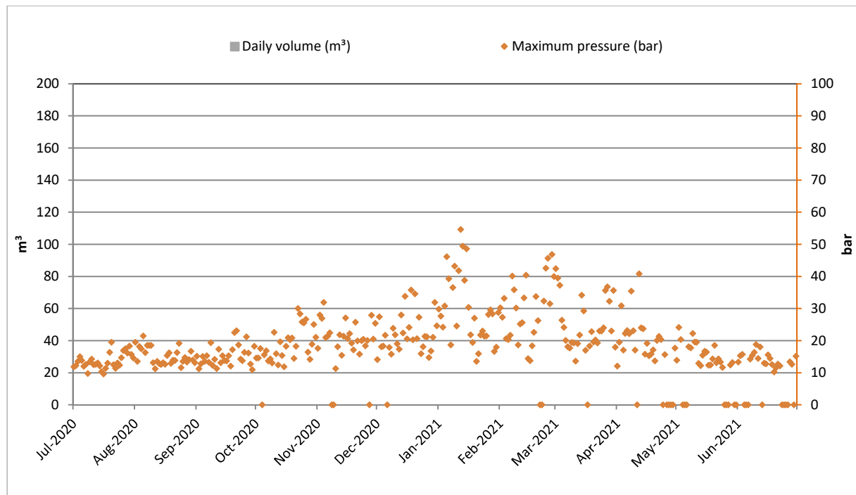
Figure 7 Manutahi-B upper daily maximum injection pressure (2020-2021)
