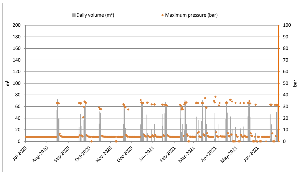
Figure 8 Manutahi-B lower daily injection and maximum pressure (2020-2021)
