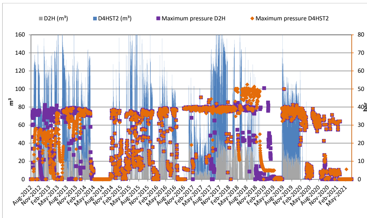
Figure 6 Manutahi-D cumulative daily injection volumes and maximum pressures (2012-2021)
