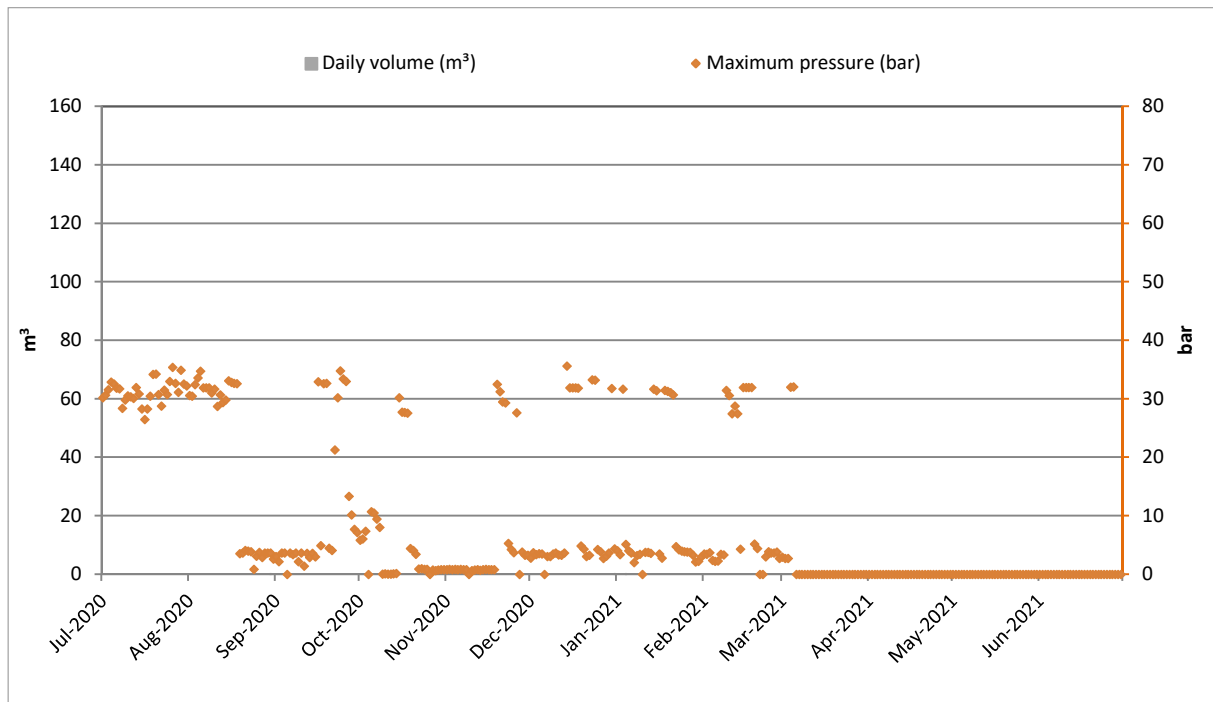
Figure 4 Manutahi-D2H daily injection volume and maximum pressure (2020-2021)
