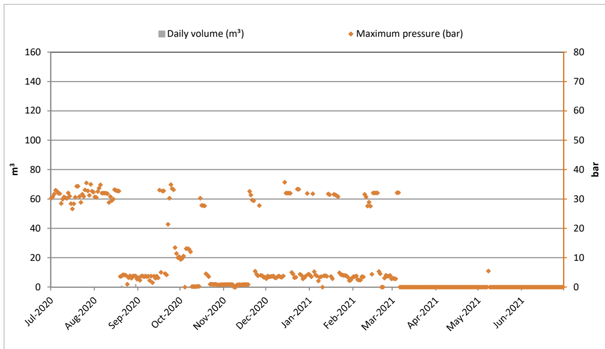
Figure 5 Manutahi-D4HST2 daily injection volume and maximum pressure (2020-2021)
