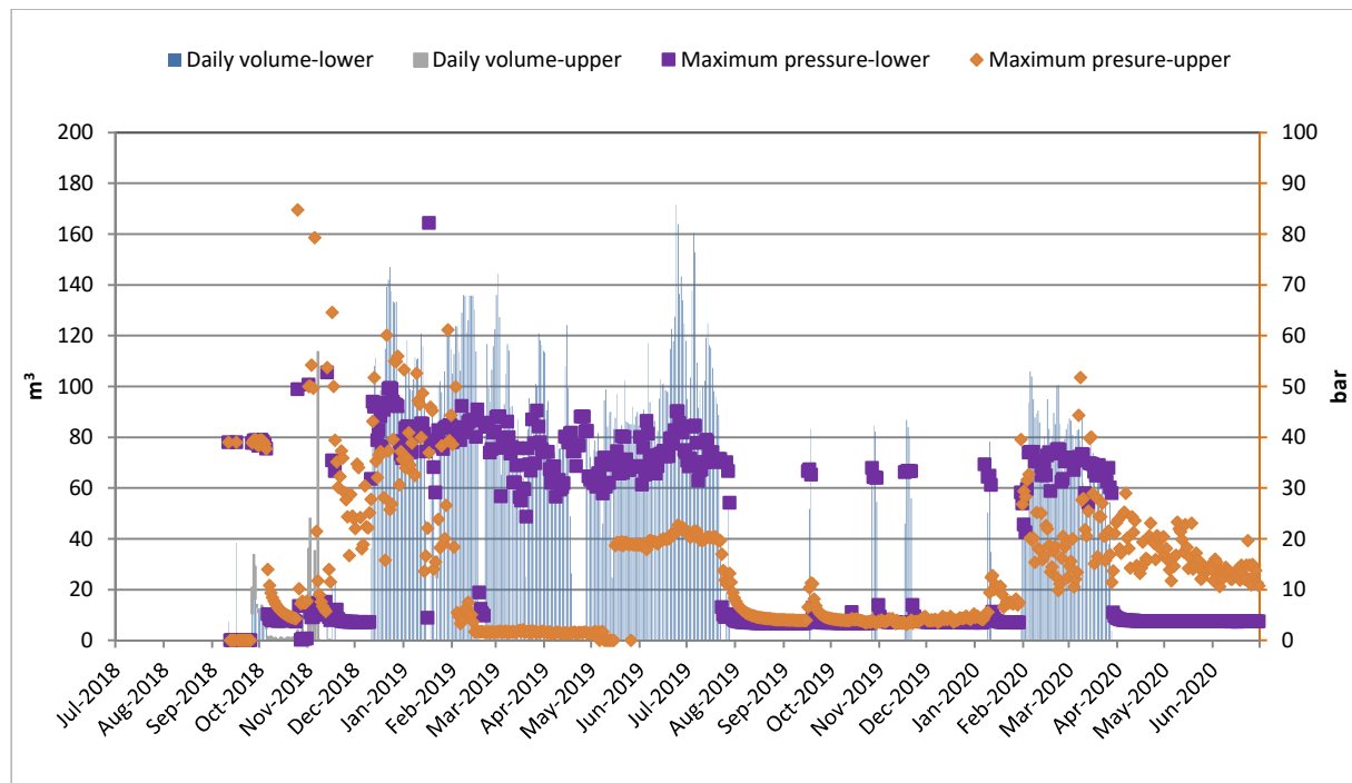
Figure 9 Manutahi-B cumulative daily injection volumes and maximum pressures (2018-2021)
