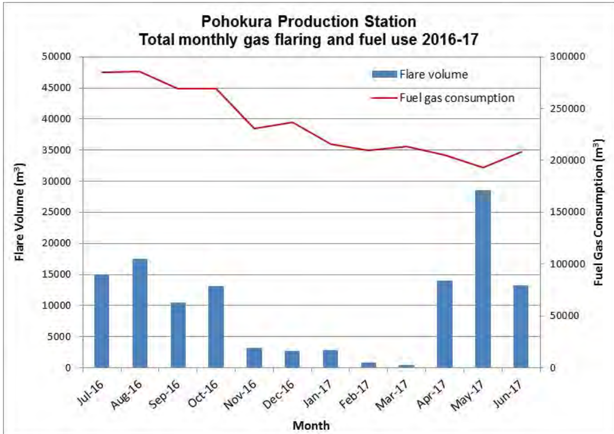
Figure 3 Monthly flare volumes and fuel gas consumption for July 2016 to June 2017
