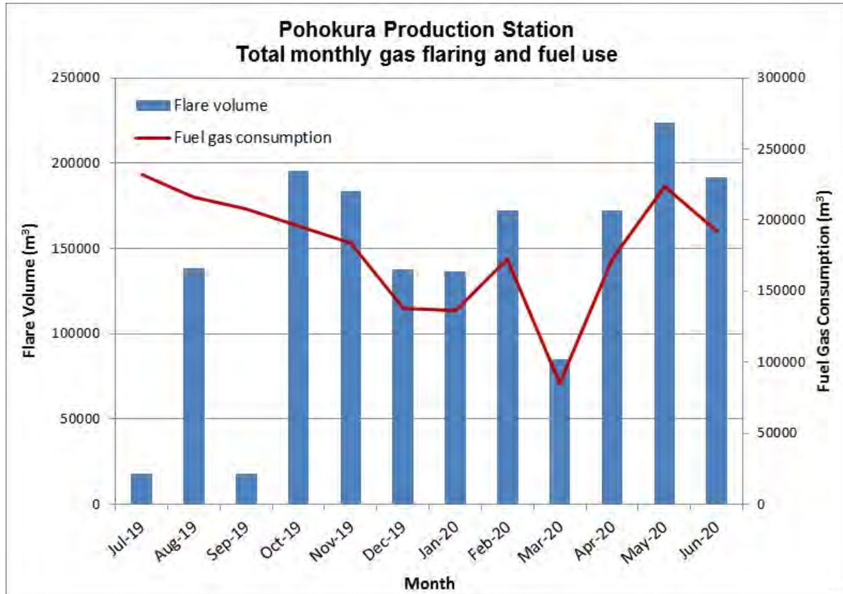
Figure 6 Monthly flare volumes and fuel gas consumption for July 2019 to June 2020
